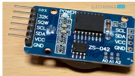
Figure 11: Real-time Clock with DS3231 Silicon Integrated Circuit
