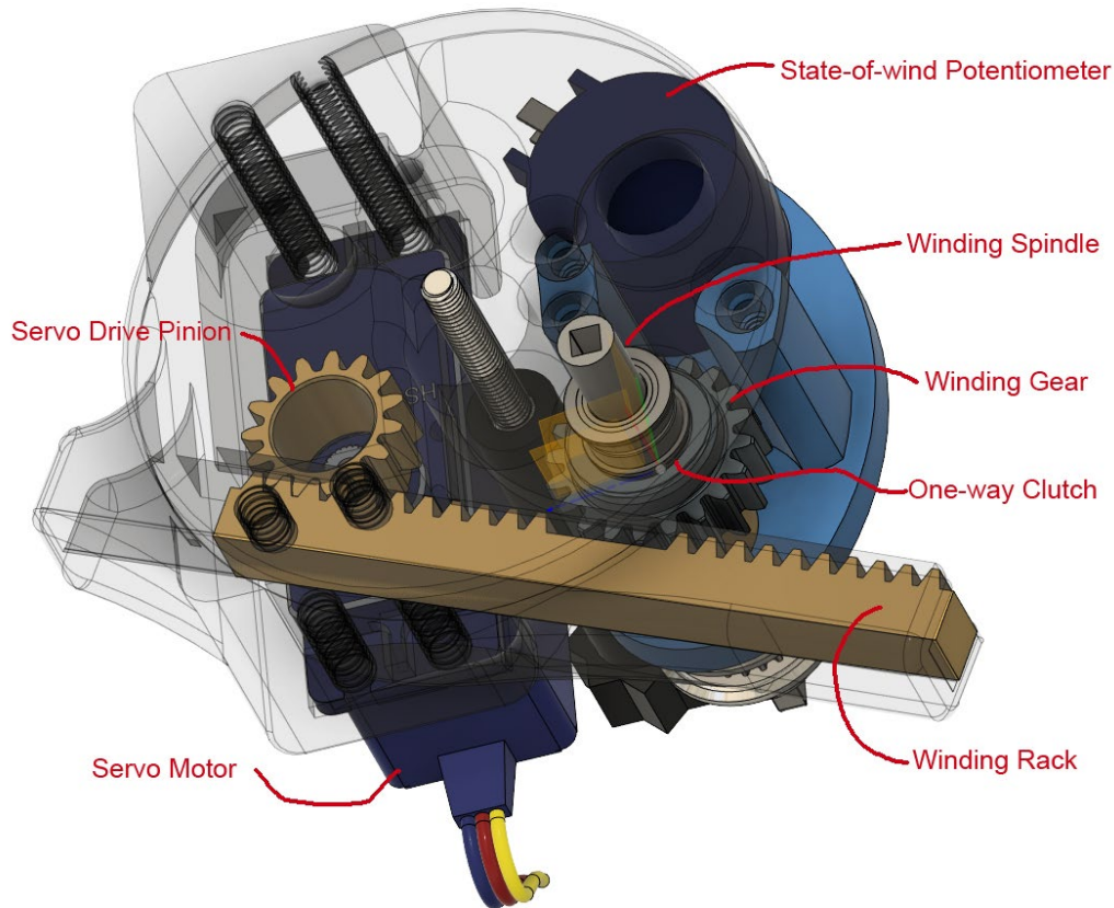
Figure 5: Winding Mechanism
