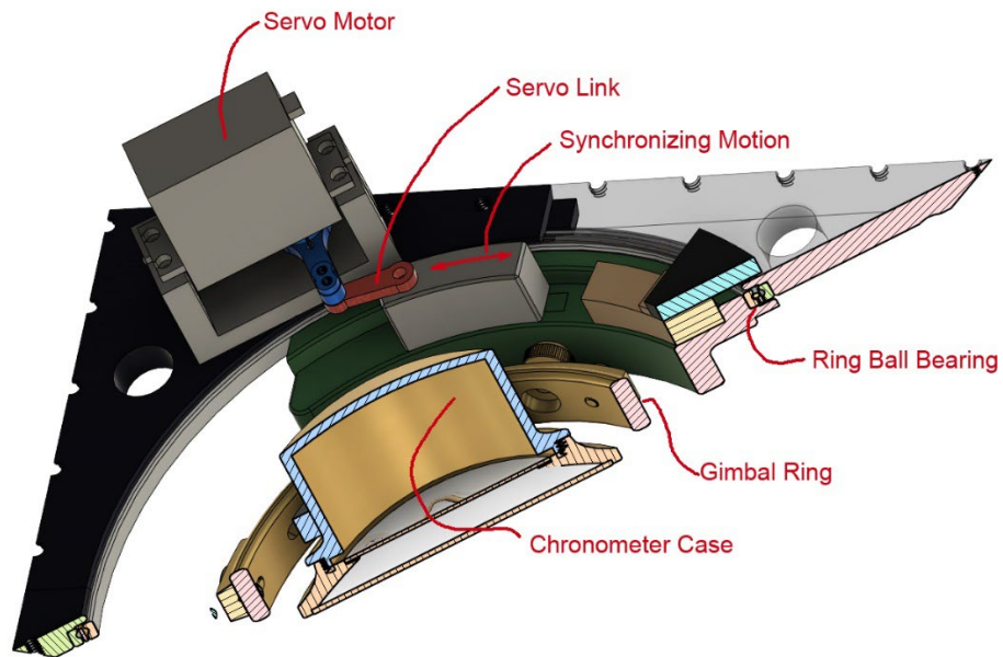
Figure 13: ServoSync Mechanism with Thin Ball Bearing Design
