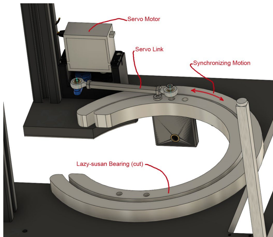
Figure 14: ServoSync Mechanism with Lazy-susan Bearing Design
